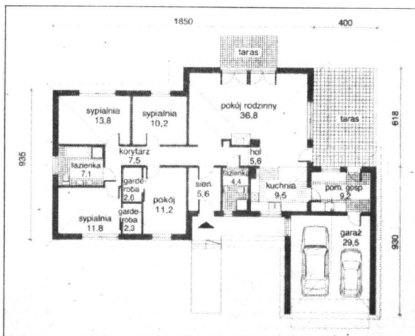
Plan parteru
